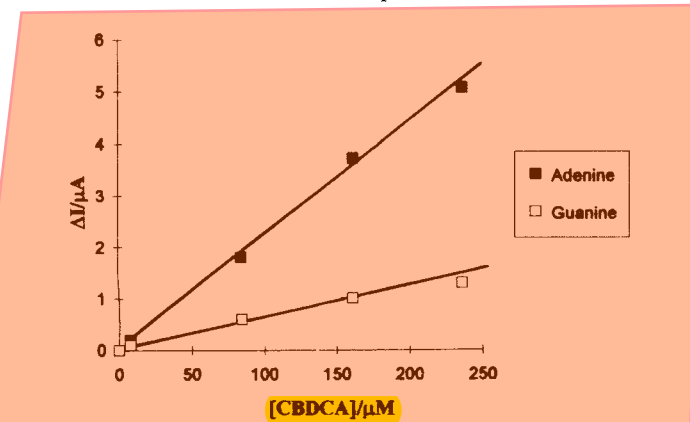
Fig. 2. Calibration plot for the decrease in the adenine (■) and guanine (□) peak current corresponding to the addition of carboplatin to a 78 \mu\text{g/mL} solution of ssDNA in pH 4.6 acetate buffer containing 0.5 mL of 5% trichloroacetic acid.
